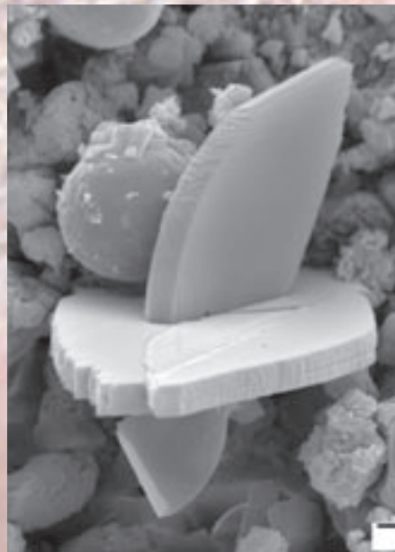
Biomineralisation products of rock eating biofilm communities on Carrara marble. The marble is eaten away and new minerals of calcium oxalate are precipitated instead. The fungal cell above the scale bar measures 3 \mu\text{m} and may have initiated a biopit.
